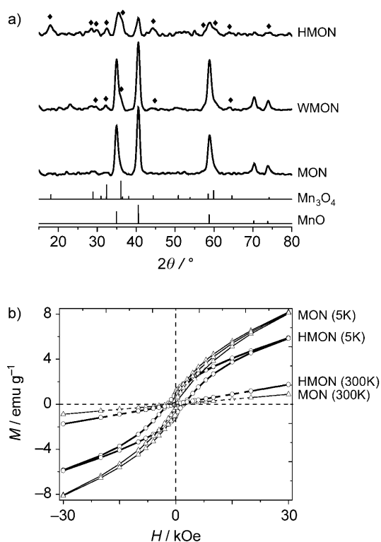
Figure 2. a) XRD patterns of MONs, WMONs, and HMIONs. Peaks corresponding to \text{Mn}_3\text{O}_4 are marked with diamonds. The lines below show the position of the reflections corresponding to cubic \text{MnO} phase (JCPDS Card No. 07-0230) and the tetragonal \text{Mn}_3\text{O}_4 phase (JCPDS Card No. 24-0734). b) Hysteresis loops of MONs ( \Delta ) and HMIONs ( \circ ) at T = 300 K (dotted lines) and T = 5 K (solid lines).
